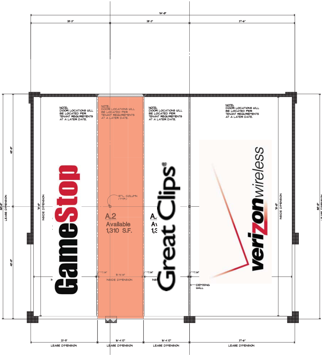
Building 'A' - Floor Plan 1/8"=1'-0"
